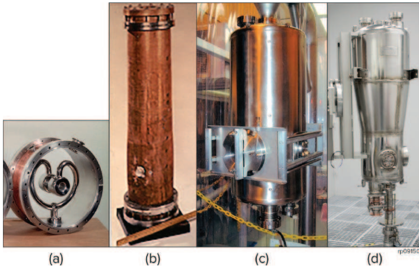
Figure 2. The photos from left to right illustrate the evolution of resonator technology developed at ATLAS: (a) the split-ring resonator first used at ATLAS, followed by various quarter-wave resonator designs used for the Positive Ion Injector in the 1990s (b), a new high-beta ( \beta = 0.13 ) design from 2008 (c), and the most recent ( \beta = 0.07 ) resonator design of 2014 (d).
