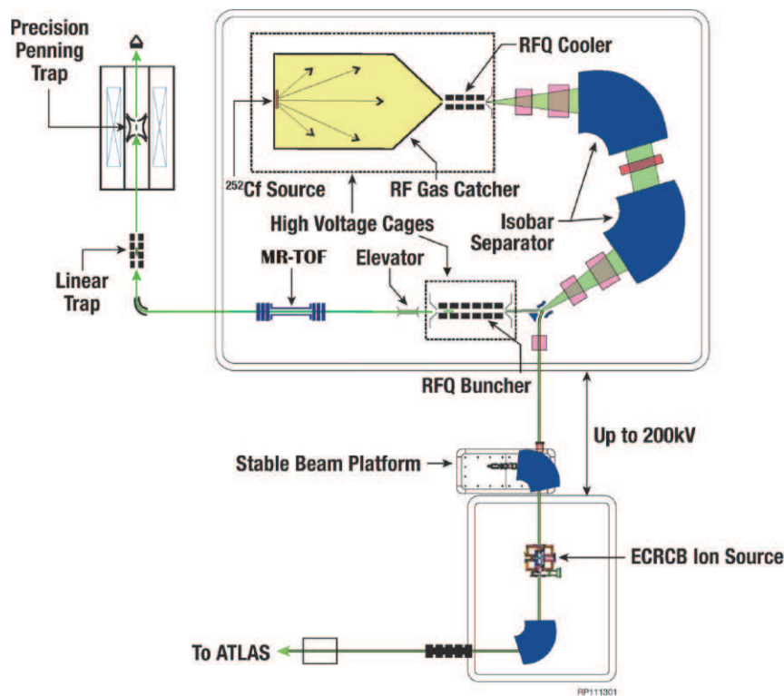
Figure 4. Floor plan of the CARIBU facility at ATLAS. The individual components are discussed in the text. The unlabeled boxes before and after the isobar separator represent quadrupole and sextupole magnets. The box between the two magnets represents an electrostatic multipole.
