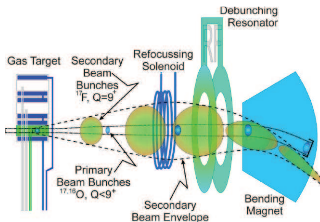
Figure 5. Principle of the in-flight technique for the production of radioactive beams.
