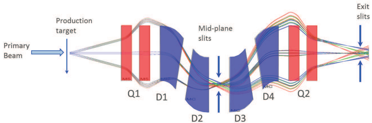
Figure 6. A schematic of the magnetic chicane now under construction for the new AIRIS in-flight facility.
