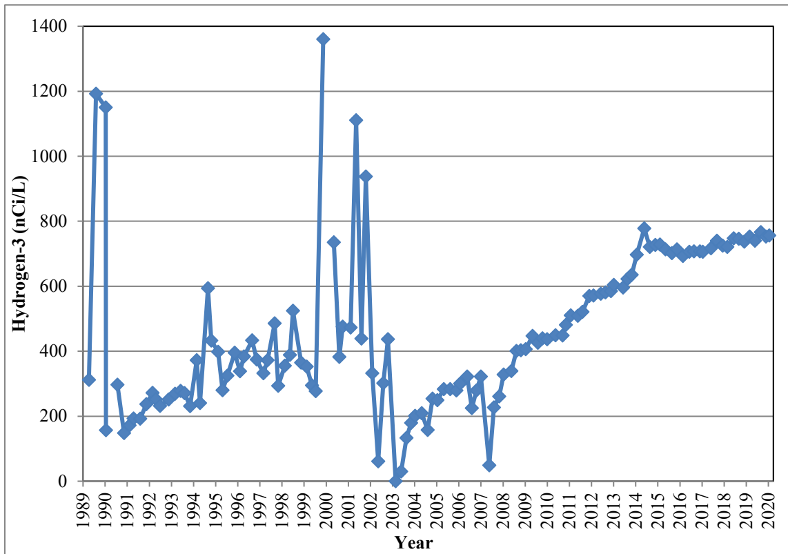
Figure 4.6 Hydrogen-3 in Well BH35
