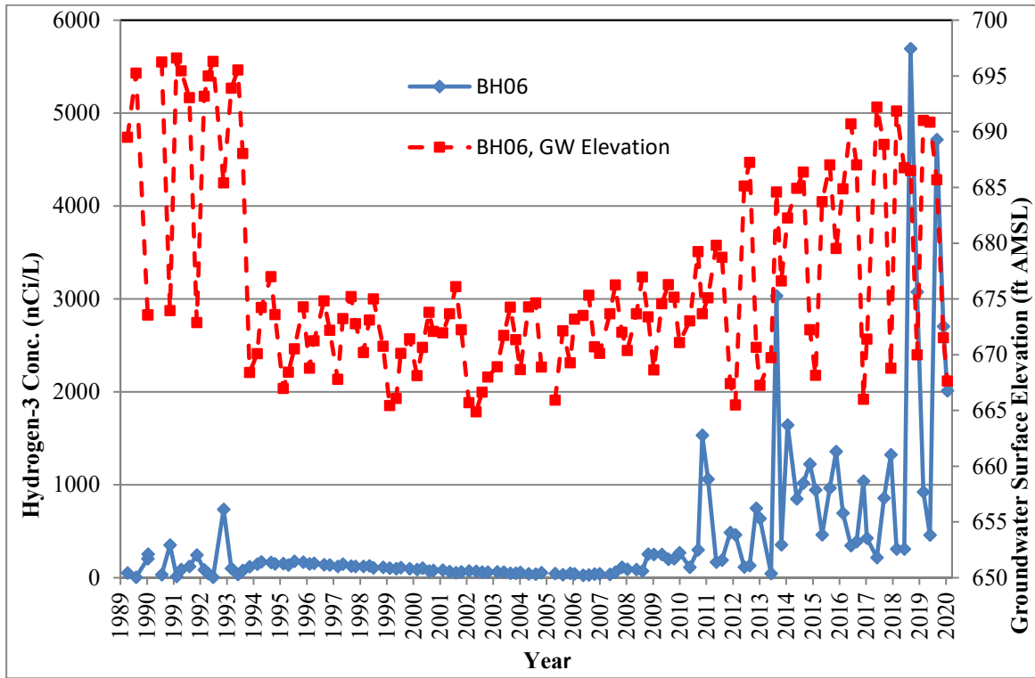
Figure 4.5 Hydrogen-3 and Groundwater Elevation in Well BH06
