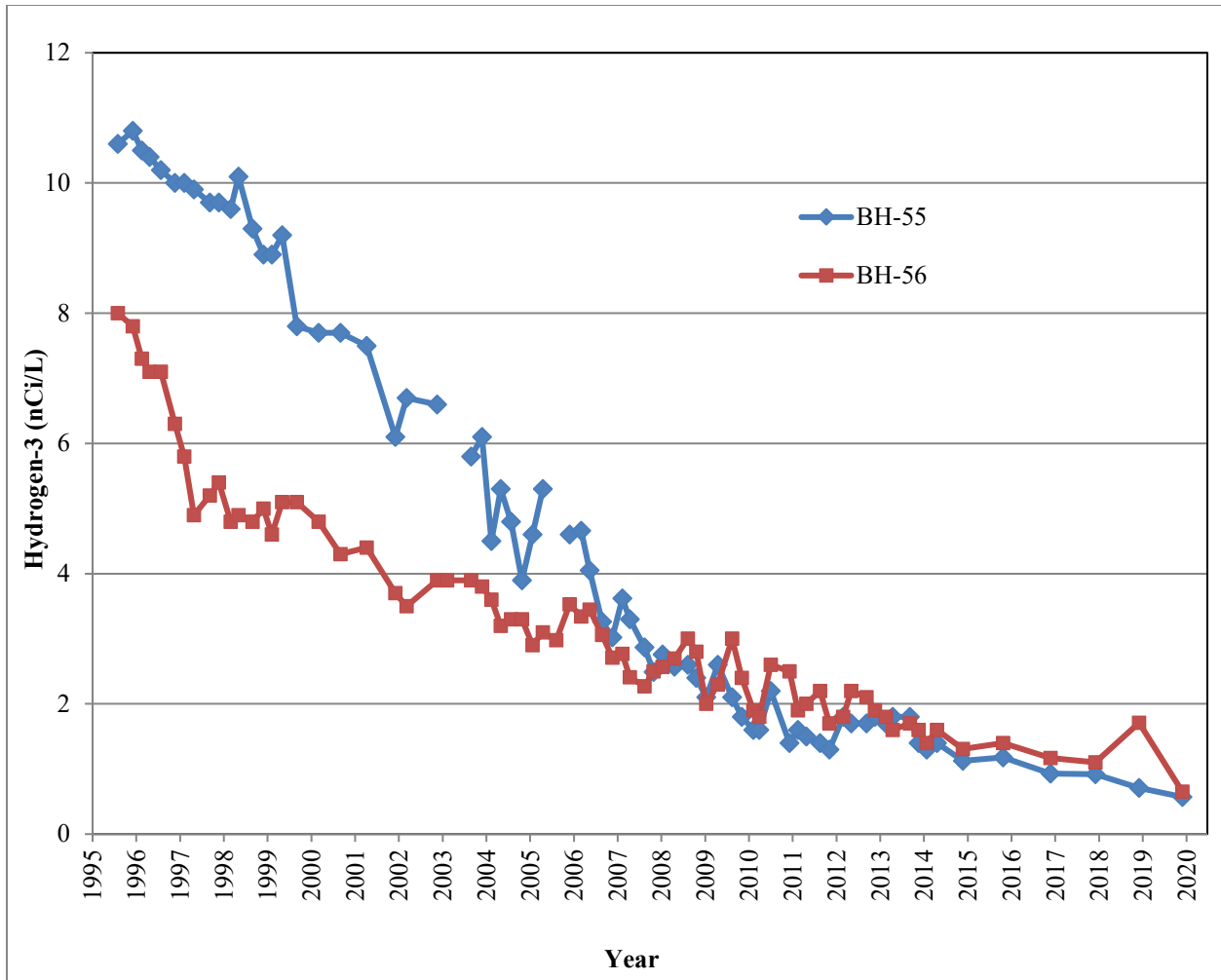
Figure 4.9 Hydrogen-3 in Site A Wells BH55 and BH56
