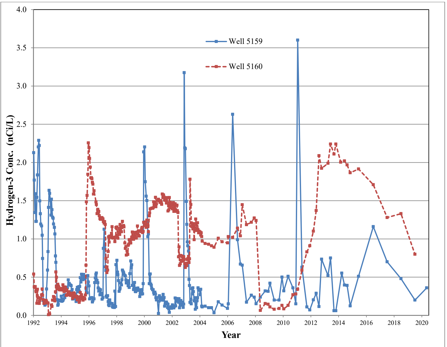
Figure 4.12 Hydrogen-3 in Former Picnic Wells from 1992 Through 2020
