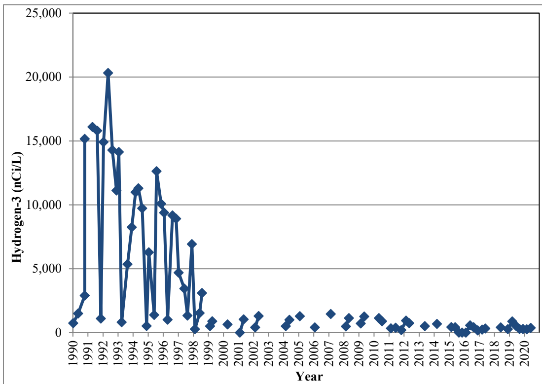
Figure 4.4 Hydrogen-3 in Plot M Well BH09
